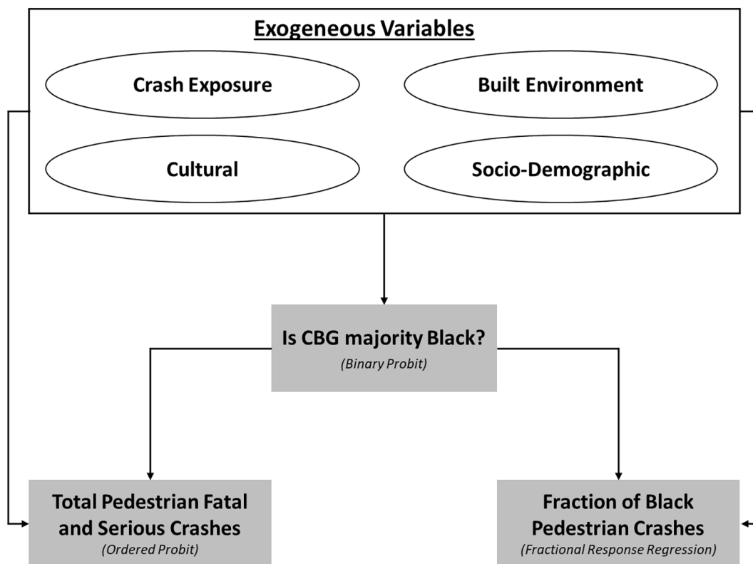
Fig. 1. Conceptual framework.
