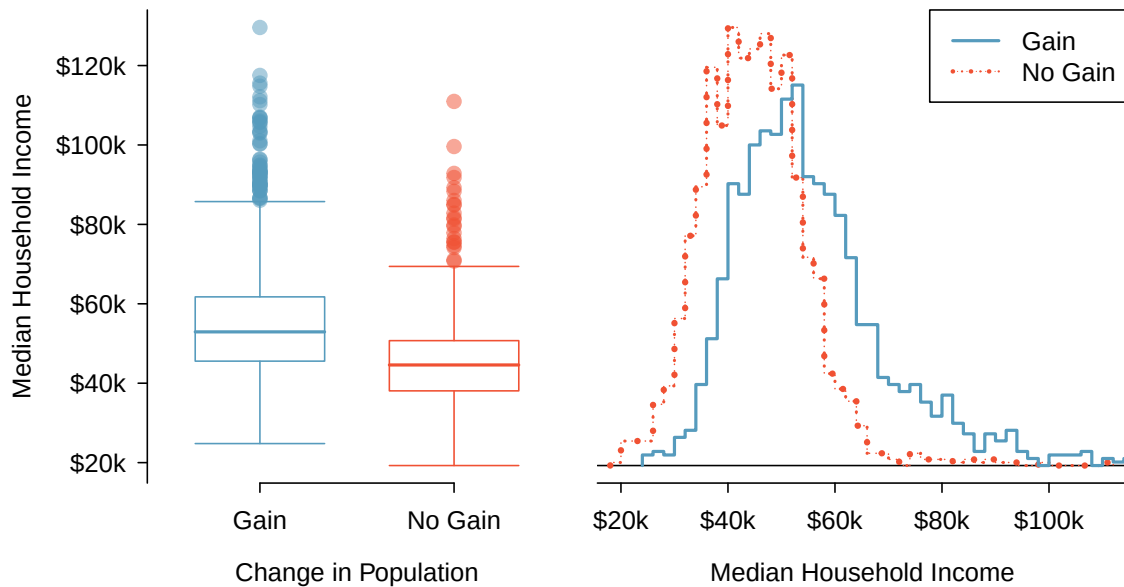
Figure 2.28: Side-by-side box plot (left panel) and hollow histograms (right panel) for med_hh_income , where the counties are split by whether there was a population gain or there was no gain.
