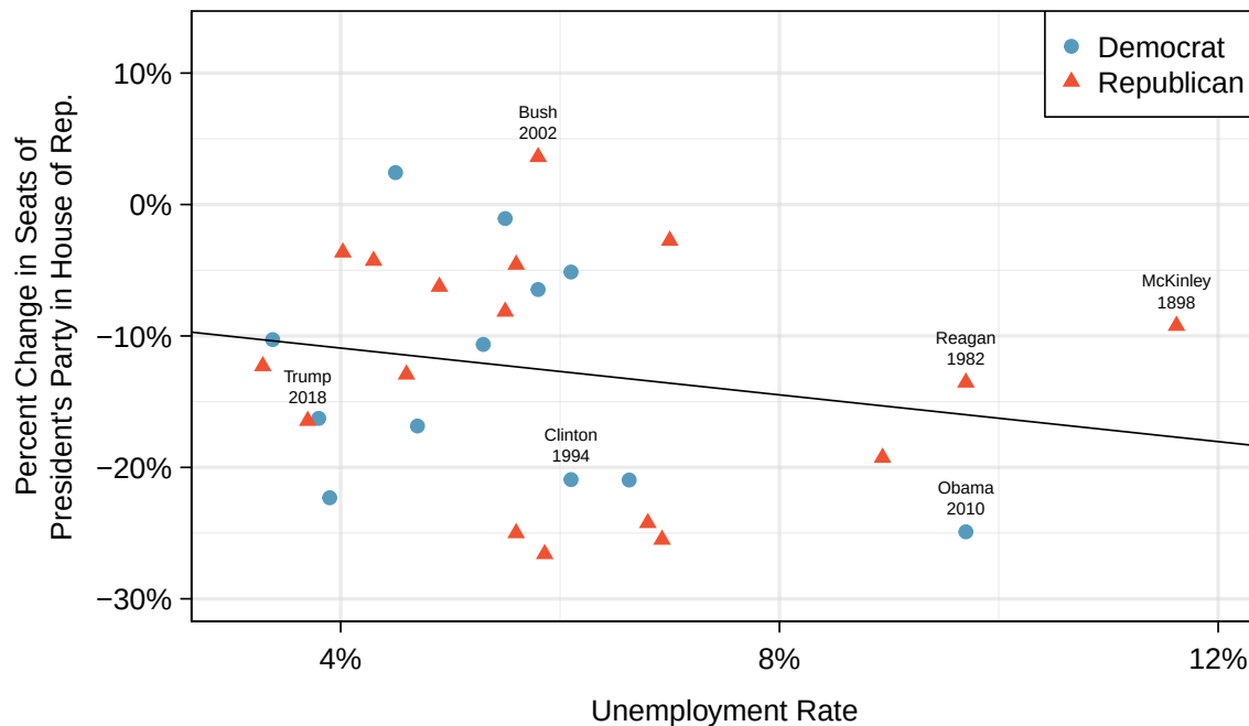
Figure 8.19: The percent change in House seats for the President's party in each midterm election from 1898 to 2018 plotted against the unemployment rate. The two points for the Great Depression have been removed, and a least squares regression line has been fit to the data.
